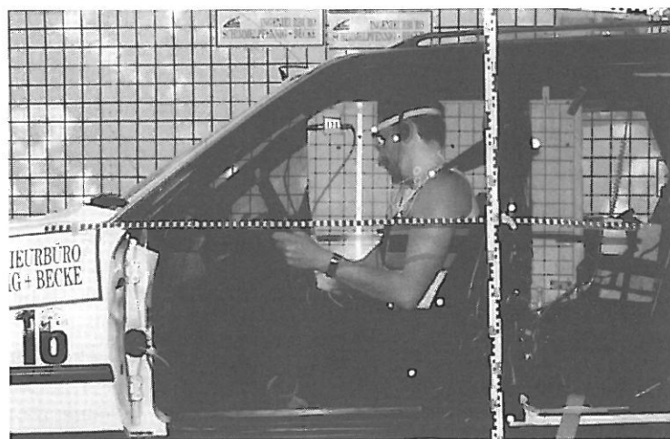
FIG. 9. Instrumentation of the occupant.
