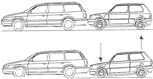
FIG. 7. Influencing factor: impact heights ( top : unbraked impact; bottom , braked impact).
