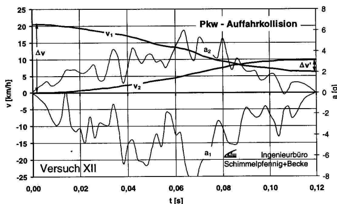
Bild 17 Pkw-Kollision Fig. 17 Vehicle rear-end collision
