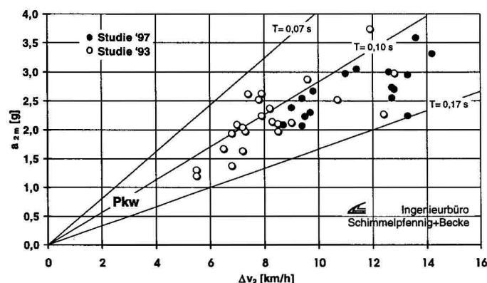
Bild 16 Meßwerte Pkw-Versuche Fig. 16 Measurement of vehicle rear-end collisions
